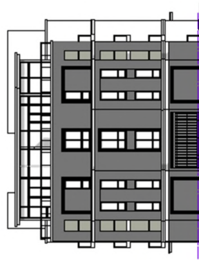
Side Elevation (West) Building D (Phase 2)
