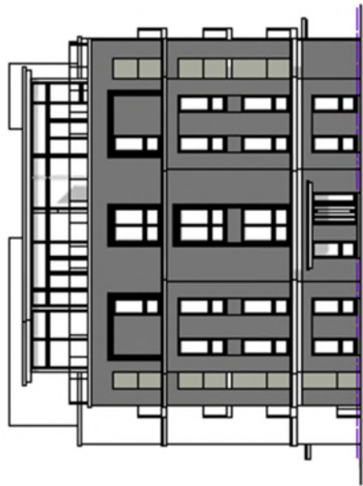
Side Elevation (East) Building D (Phase 2)
