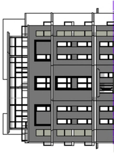
Side Elevation (West) Building C (Plan 34-02)
